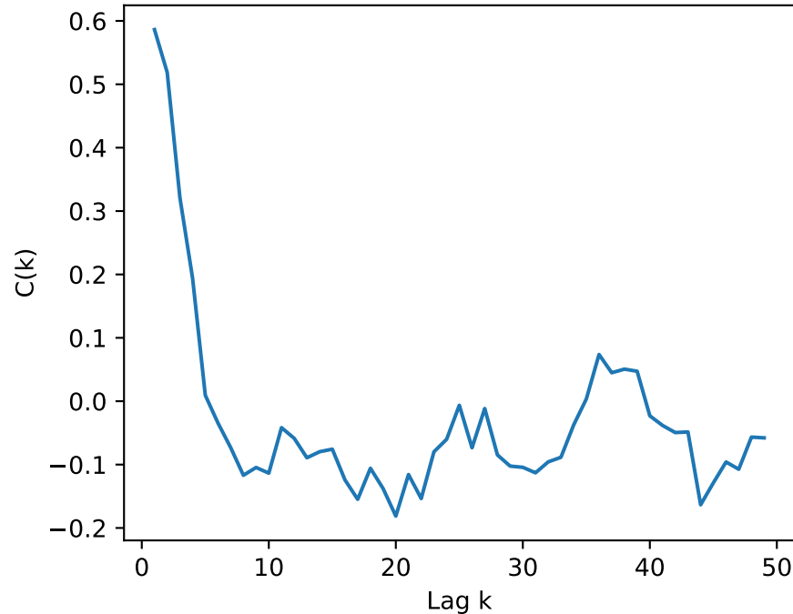
HOMO Autocorrelation
