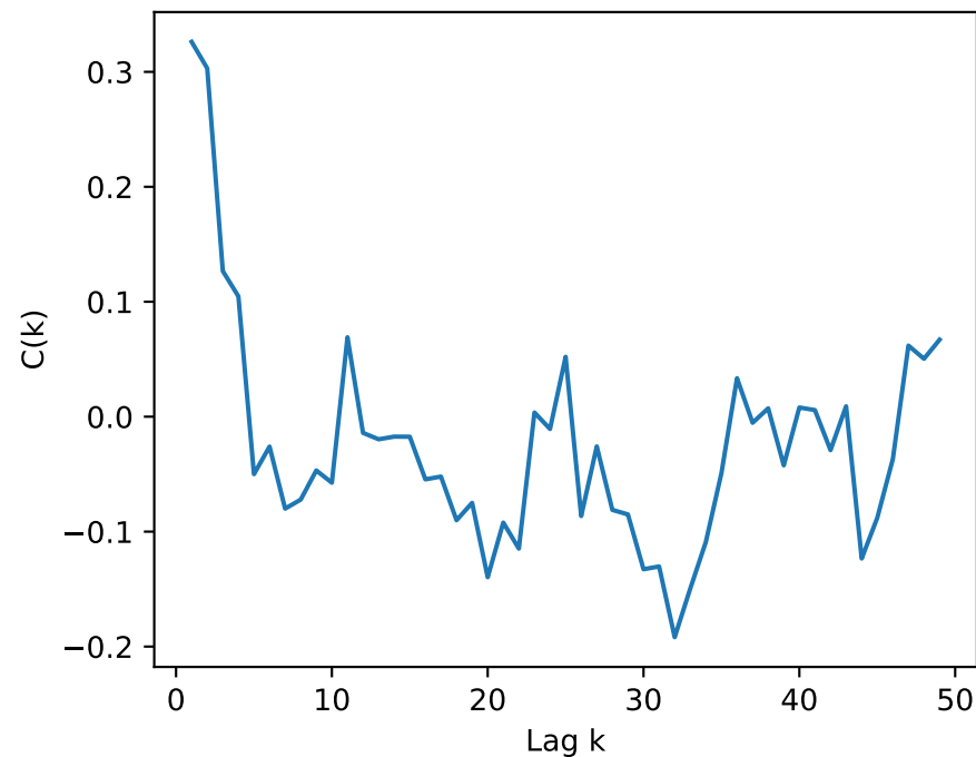
GAP Autocorrelation
