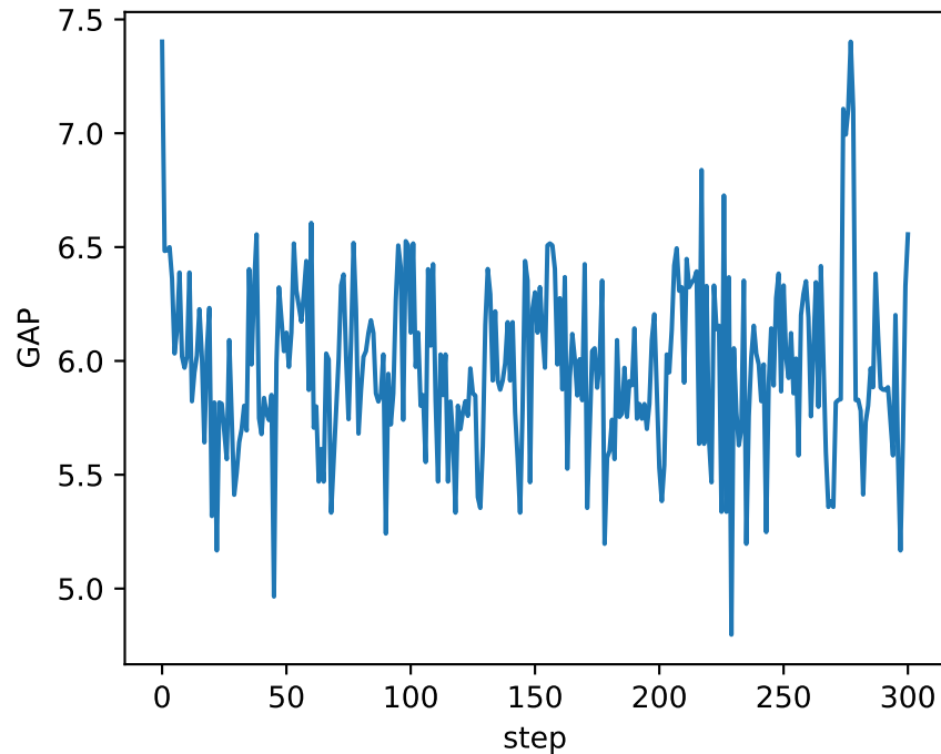
GAP - evolution
