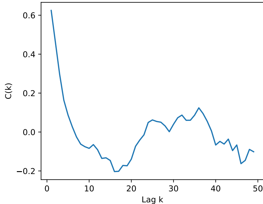
LUMO Autocorrelation
